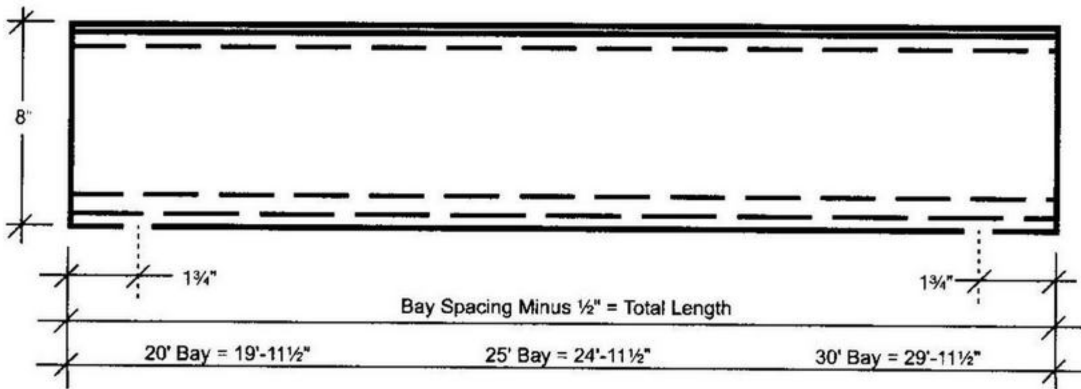
FLANGE PUNCHING SIDE VIEW
