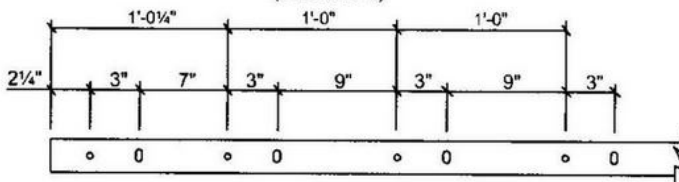
Pattern D & E - Common Flange
