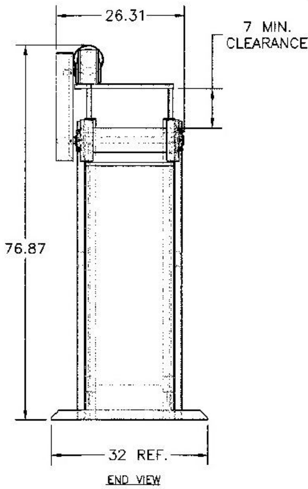
END VIEW
