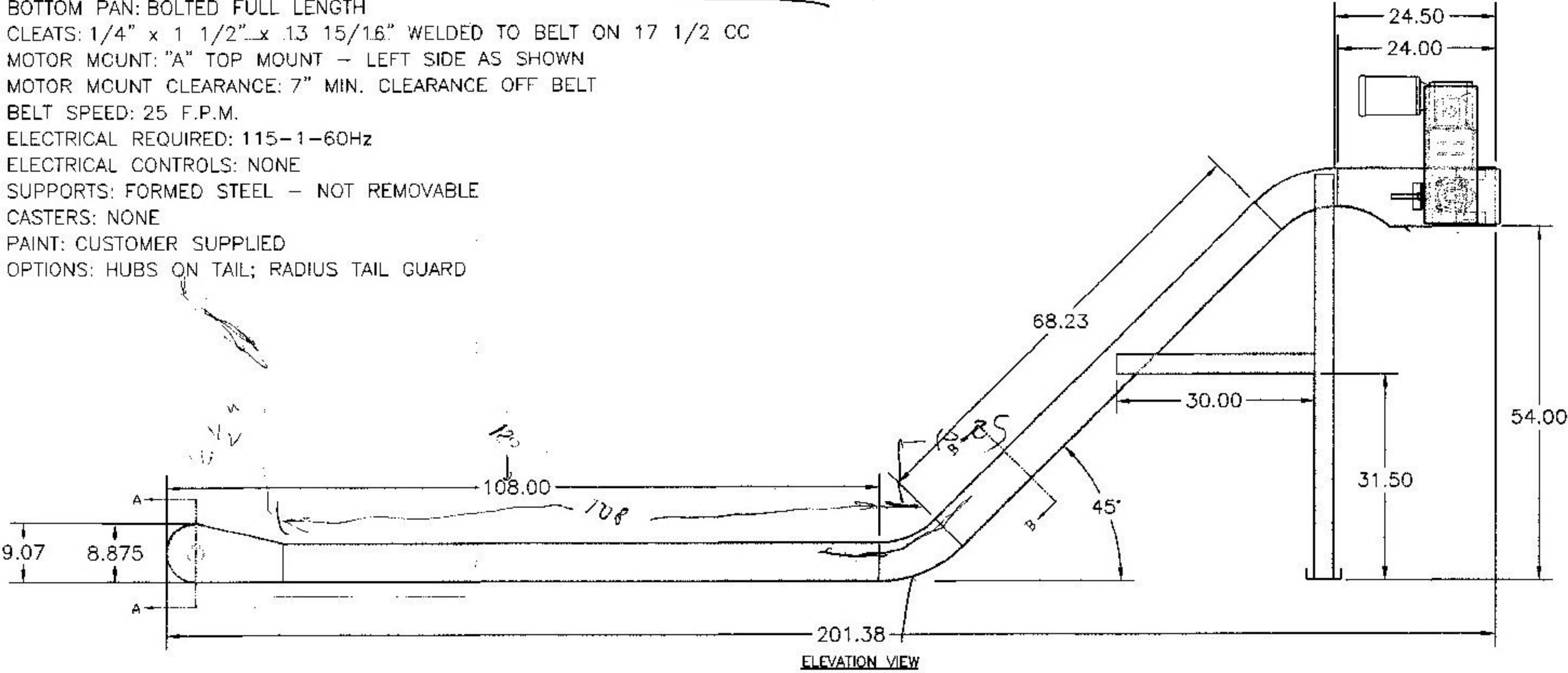
ELEVATION VIEW
