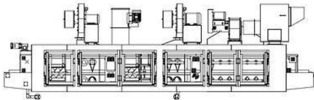
FRONT
